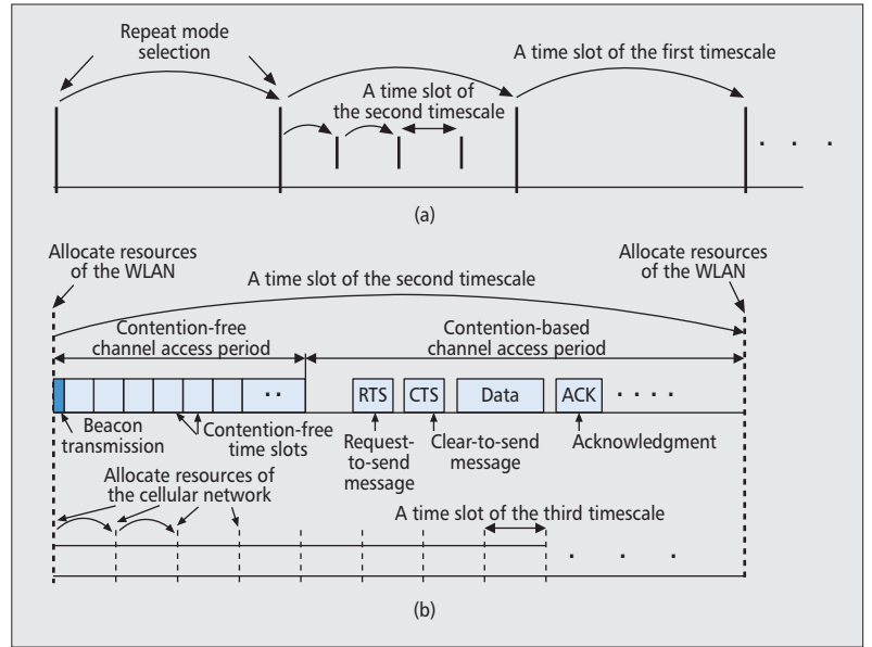
Figure 3. Proposed three-timescale resource allocation scheme: a) operations of the first and second timescales; b) detailed view of a second timescale time slot.
