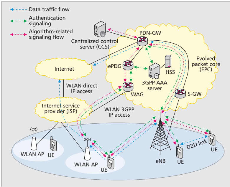
Figure 5. Semi-distributed implementation of the proposed resource allocation scheme.
