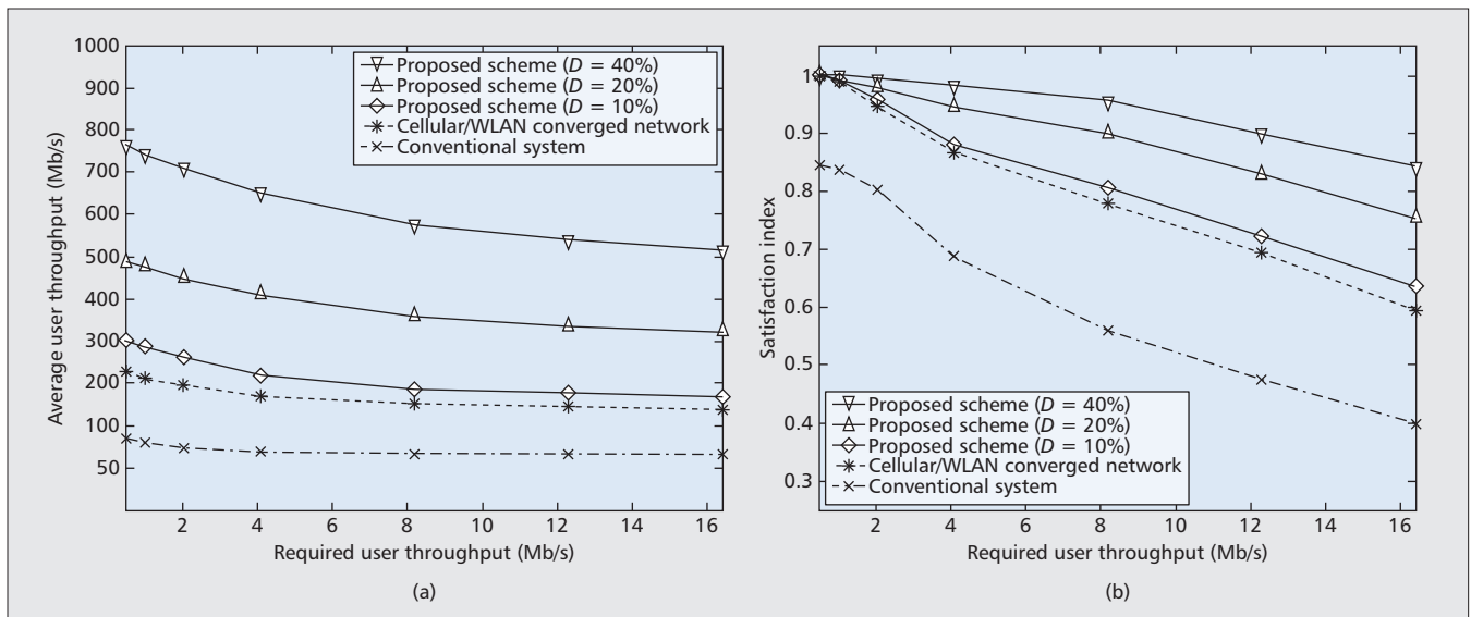
Figure 6. Performance comparison: a) throughput performance; b) QoS satisfaction.
