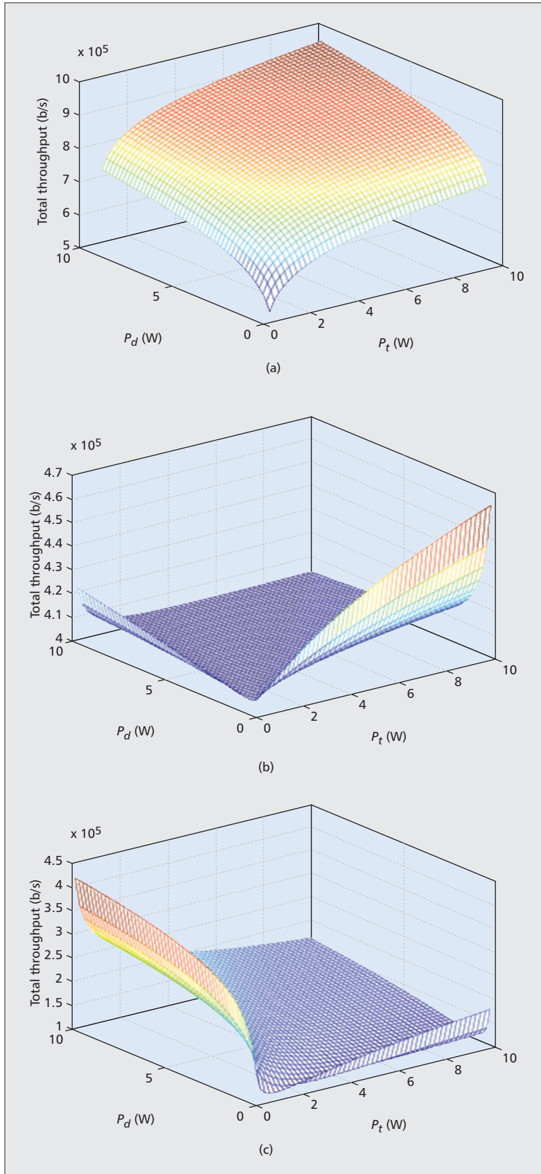
Figure 2. Throughputs achieved reusing a RB for a D2D and a traditional link: a) D2D and traditional links are far away from each other; b) two links are in proximity, and the traditional link has a higher channel gain; c) two links are in proximity, and the D2D link has a higher channel gain.
