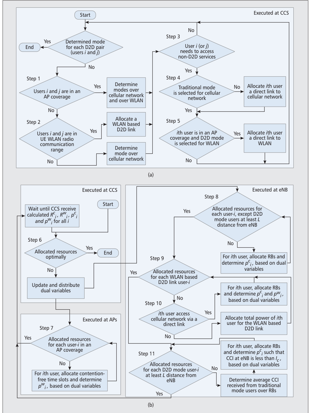
Figure 4. a) Mode selection algorithm; b) second timescale joint resource allocation algorithm.
