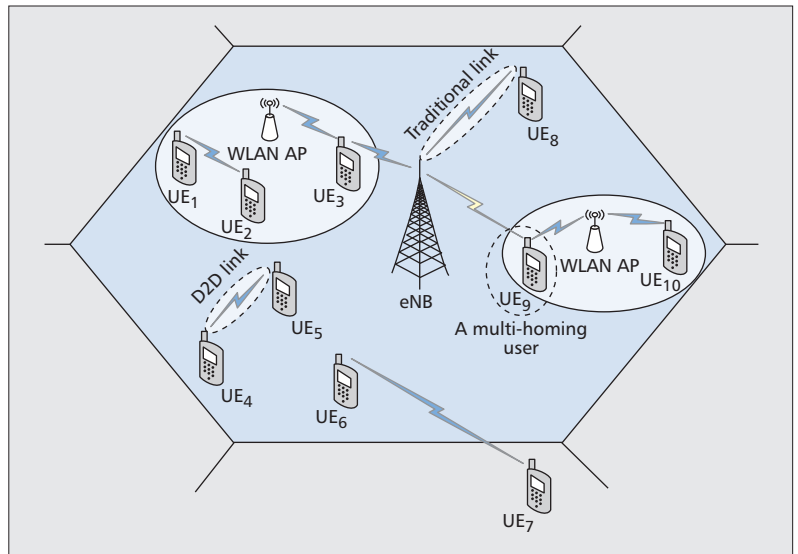
Figure 1. Underlying cellular/WLAN converged D2D communication network.
