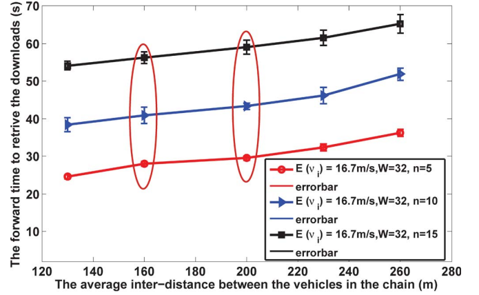
Fig. 20. Effect of intervehicle distance for data forward delay.
