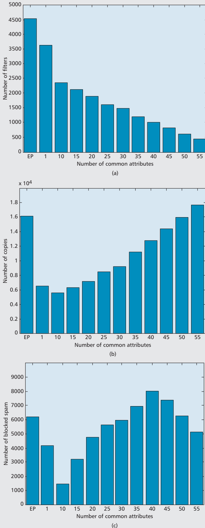
Figure 5. Performance comparison. EP denotes the epidemic filter distribution (distribute to every encountered user). TH is the number of common attributes between the filter creator and the holders: a) number of filters vs. TH; b) number of copies vs. TH; c) number of blocked packets vs. TH.
