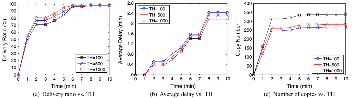
Fig. 6. Impact of TH on performance of PHDA.
