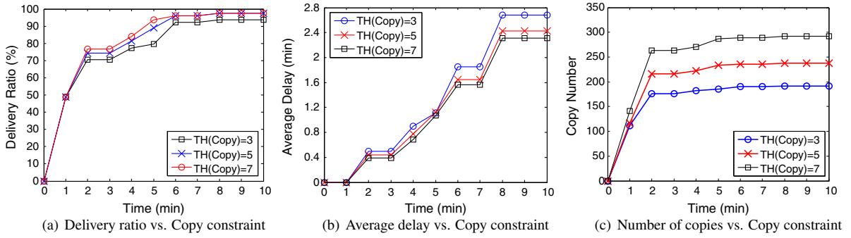
Fig. 5. Impact of copy constraints on performance of PHDA.
