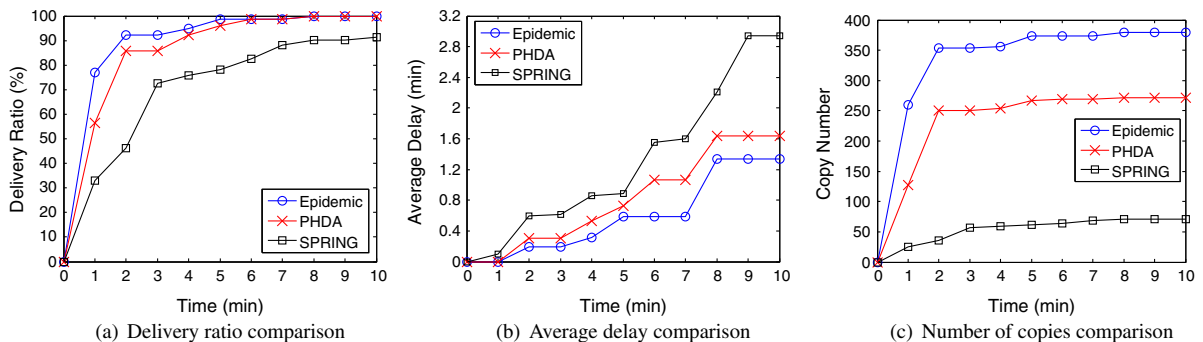
Fig. 4. Emergency call performance between PHDA and epidemic.
