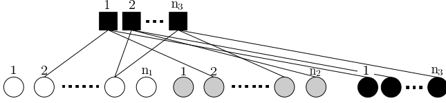
Fig. 5. The equivalent graph of the systematic LDPC code at the relay node.
