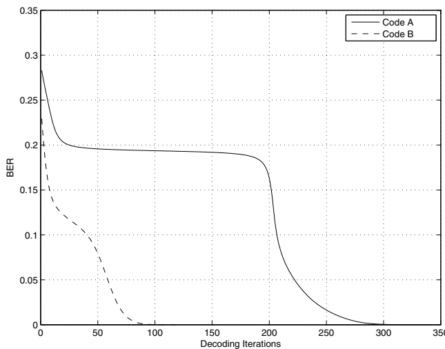
Fig. 9. Evolution of the bit error rate during iterative decoding.
