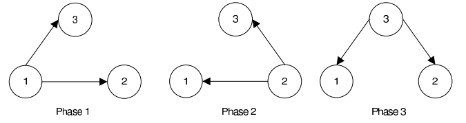
Fig. 1. Three phases in half-duplex two-way relay channels.
