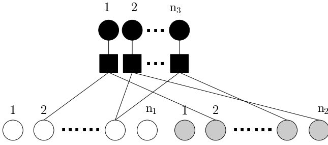
Fig. 4. The graph of the systematic LDPC code at the relay node.
