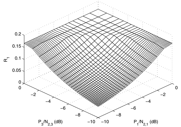
Fig. 2. Achievable rates of R_1 for \left( \frac{P_1}{N_{2,1}}, \frac{P_3}{N_{2,3}} \right) pairs.
