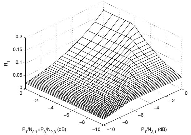
Fig. 3. Achievable rates of R_1 for \left( \frac{P_1}{N_{3,1}}, \frac{P_1}{N_{2,1}} \left( \frac{P_3}{N_{2,3}} \right) \right) pairs.
