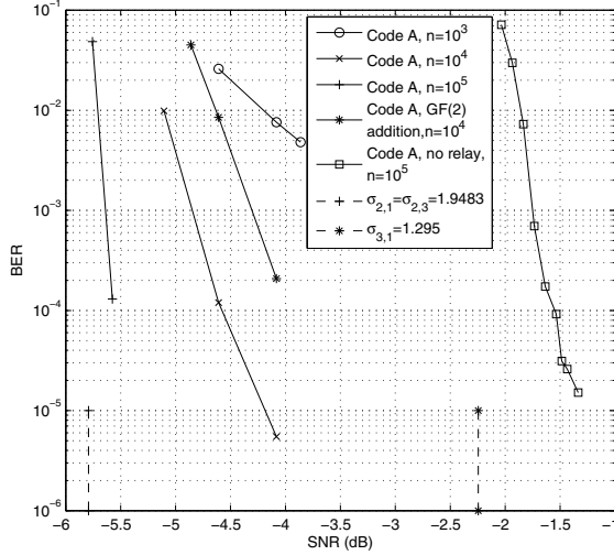
Fig. 7. Simulation results when decoding code A at terminal node 2.
