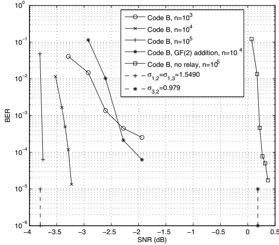
Fig. 8. Simulation results when decoding code B at terminal node 1.
