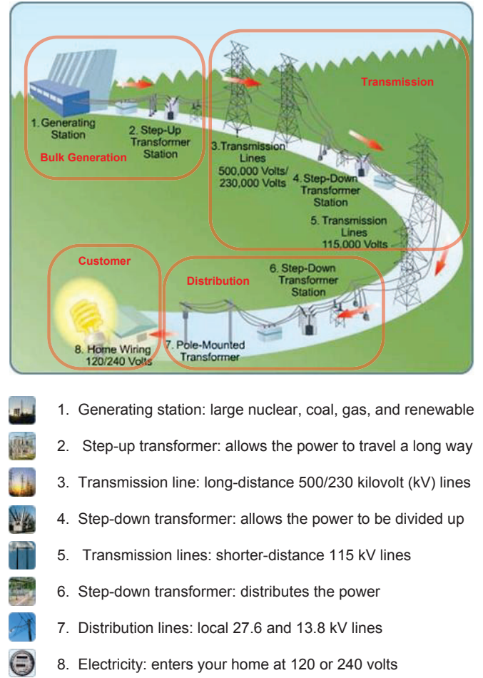
Fig. 8. An overview of bulk generation and transmission systems [60].
