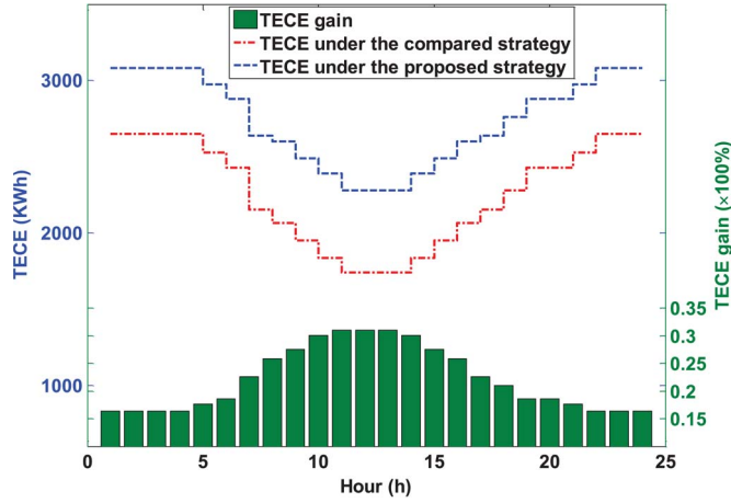
Fig. 8. Daily TECE comparison when the total number of EVs is fixed to 1200.
