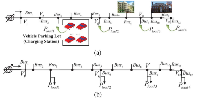
Fig. 2. The power system model. (a) Illustrated power system model. (b) Equivalent power system.
