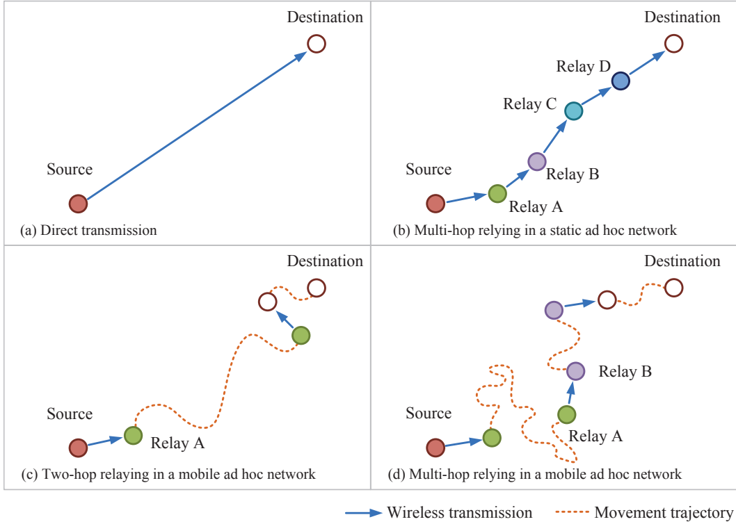
Fig. 3. An illustration of packet transmission strategies.
