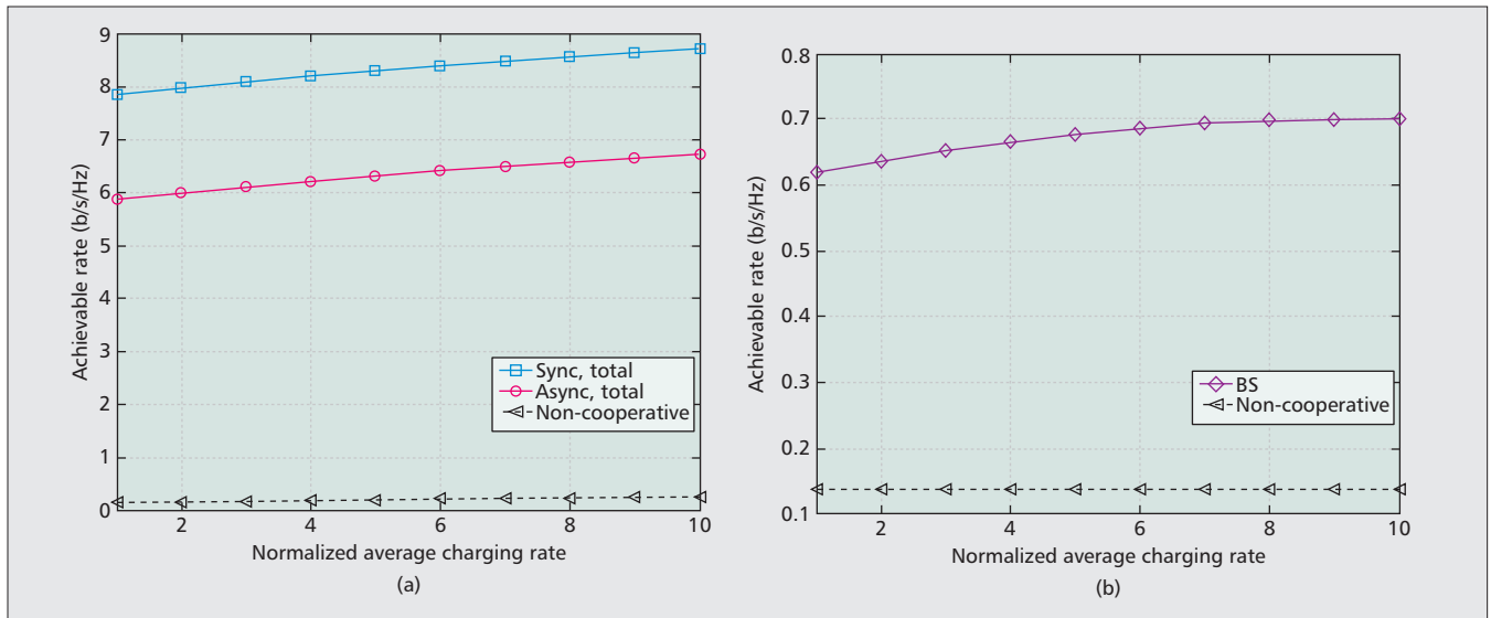
Figure 4. Rate comparison under various charging rate: a) total power constraint; b) BS power constraint.
