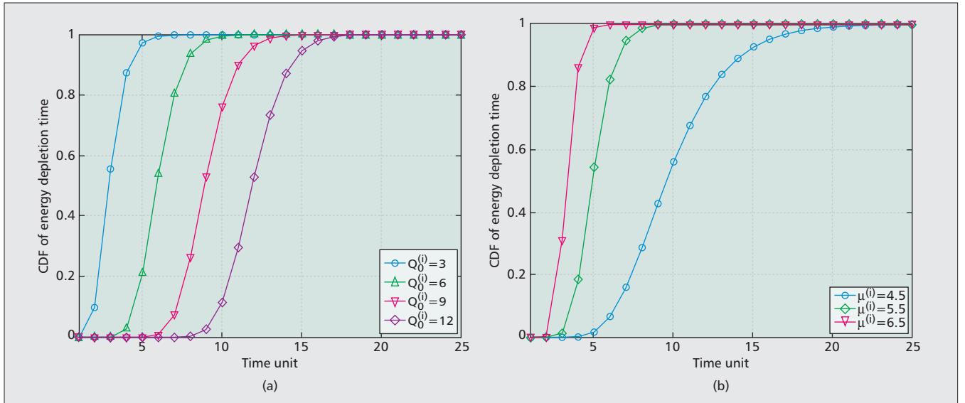
Figure 3. CDF of energy depletion time: a) \lambda^{(i)} = 3.5, \mu^{(i)} = 5.5 ; b) Q_0^{(i)} = 10, \lambda^{(i)} = 3.5 .
