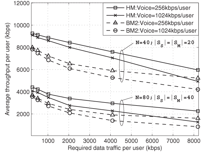
Fig. 7. Throughputs achieved by different algorithms in system-2.
