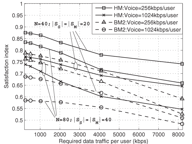
Fig. 9. Satisfaction index achieved by different algorithms for data traffic in system-2.
