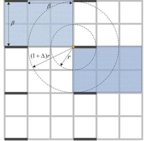
Fig. 7. Example of noninterfering transmission group of road segments.
