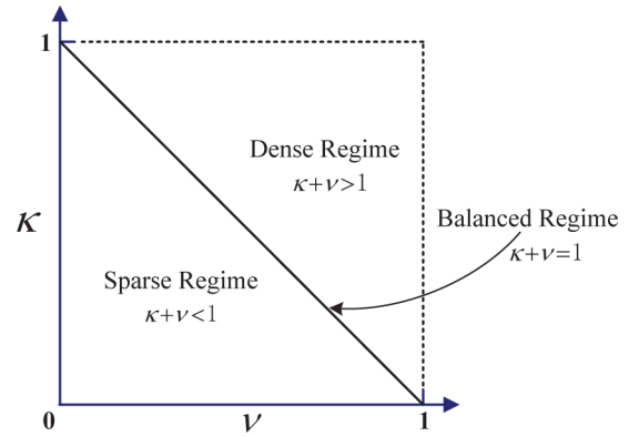
Fig. 4. Regimes for asymptotic performance limits with respect to \kappa and \nu .
