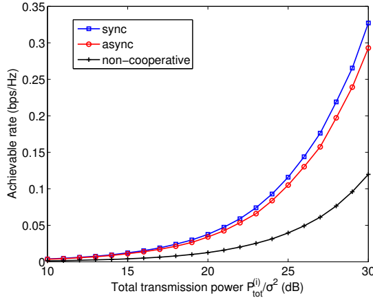
Fig. 2. Rate comparison under the total power constraint for a single-user channel.
