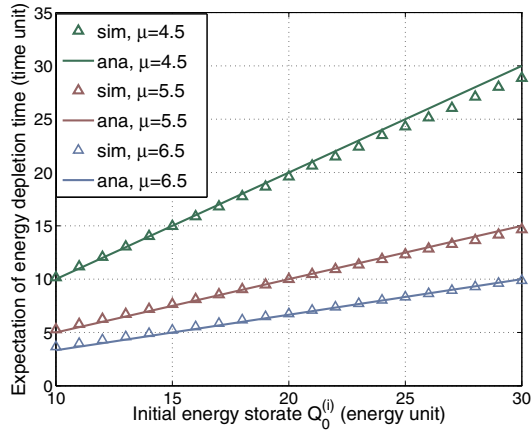
Fig. 5. Expectation of depletion duration ( \lambda^{(i)} = 3.5 ).
