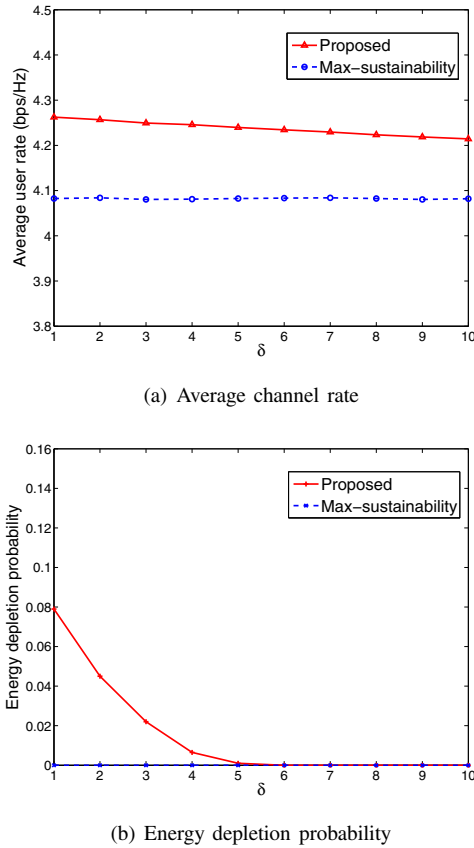
Fig. 7. BS power constraint case (channel number=20, P_s = 2\text{dB} ).
