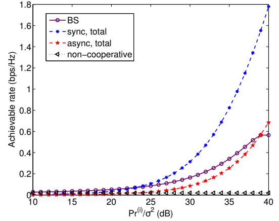
Fig. 3. Rate comparison for a single-user channel.
