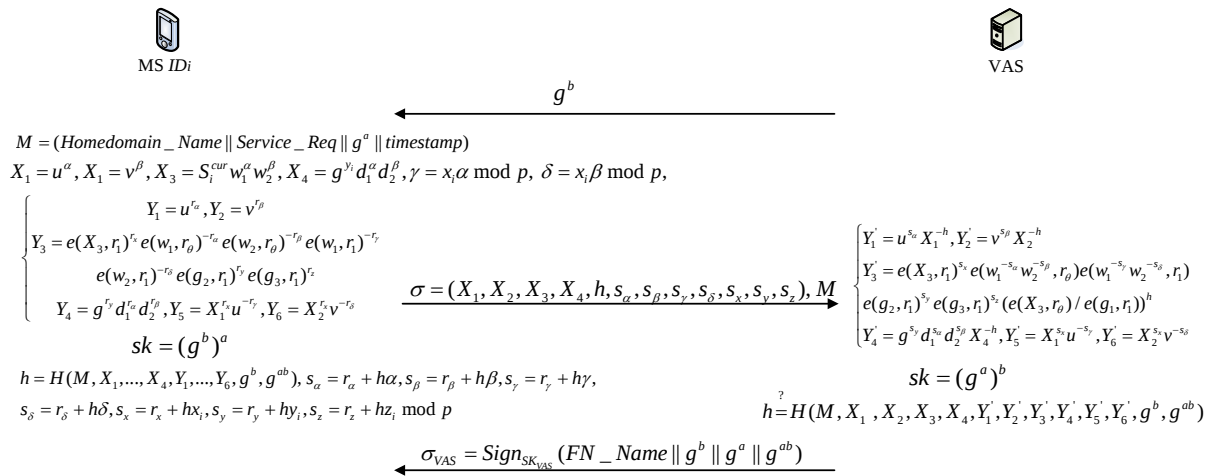
Fig. 3. The access authentication between the MS and the VAS during roaming
