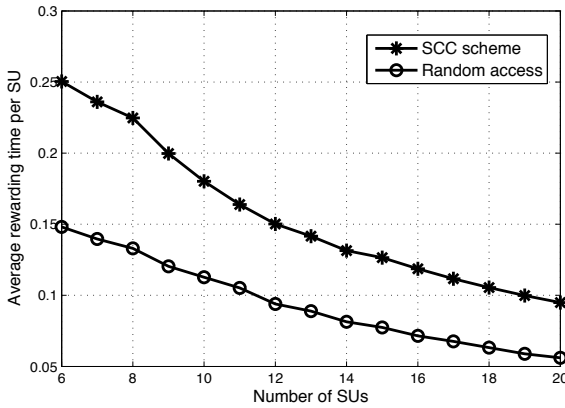
Figure 8. Average access time per SU averaged over fading for SCC scheme and random channel access
