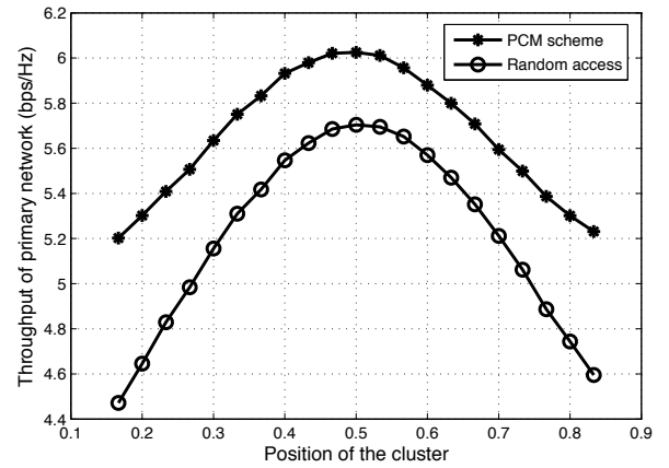
Figure 6. Throughput of the primary network, averaged over fading, versus the position of the cluster
