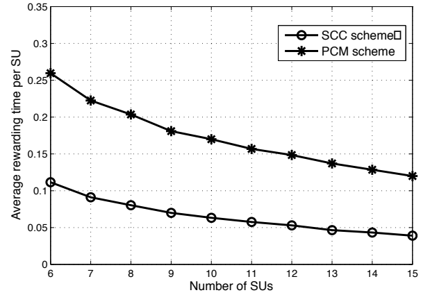
Figure 10. Average access time per SU averaged over fading for PCM scheme and SCC scheme
