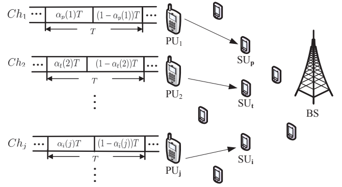
Figure 1. Cooperative cognitive radio network with multiple channels
