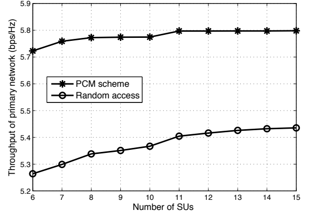
Figure 5. Throughput of the primary network averaged over fading versus number of SUs
