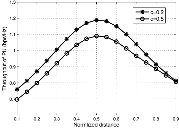
Figure 2. Throughput of PU, averaged over fading, versus the normalized distance d .
