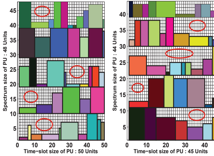
Fig. 4. The packing result by random packing strategy.
