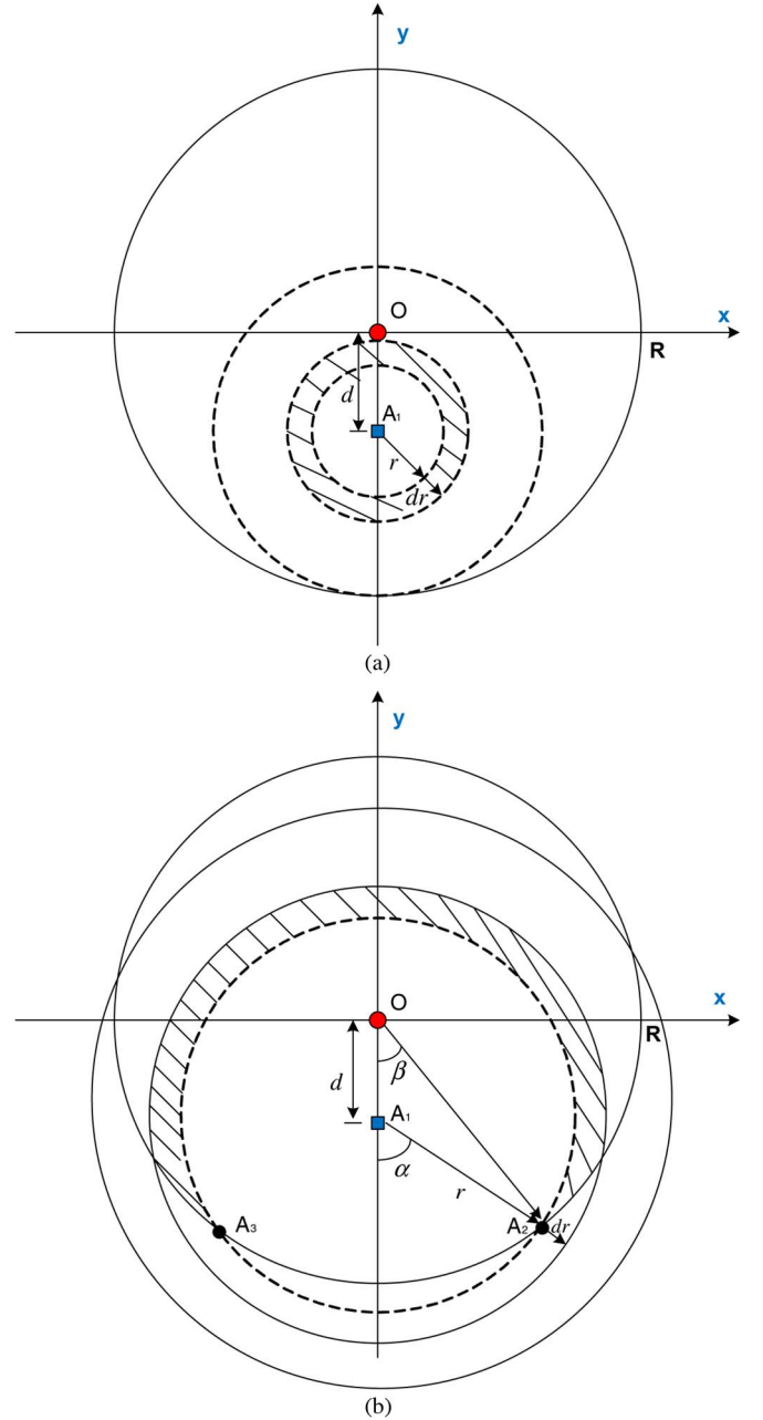
Fig. 3. Geometric illustration for evaluation of P_{e1} . (a) Case 1: r \leq R - d . (b) Case 2: r \geq R - d .
