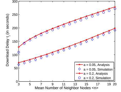
Fig. 10. Mean file download delay with different values of \langle n \rangle
