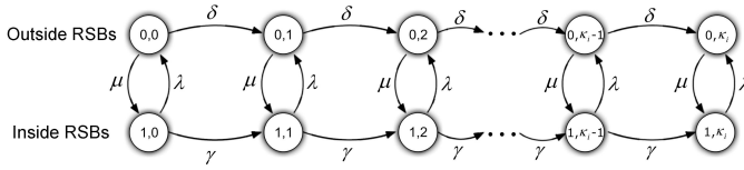
Fig. 2. State space and transitions of the two-dimensional Markov process
