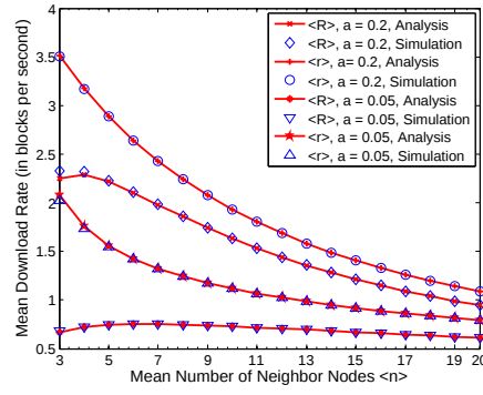
Fig. 9. Mean download rate with different values of \langle n \rangle
