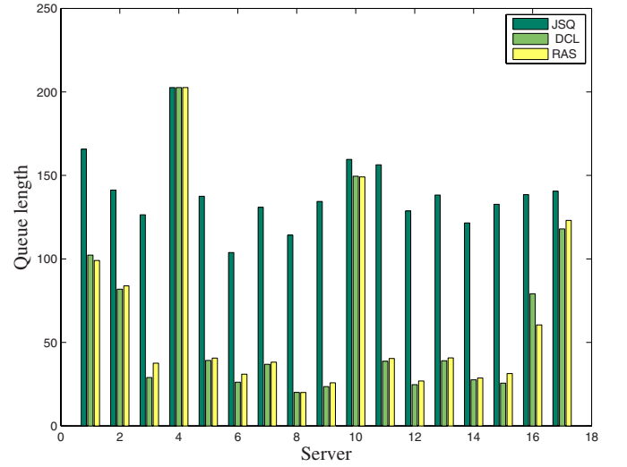
Fig. 6. Comparison of average queue length of JSR, DCL, and RAS.
