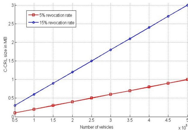
Fig. 5: C-CRL size versus the number of vehicles.
