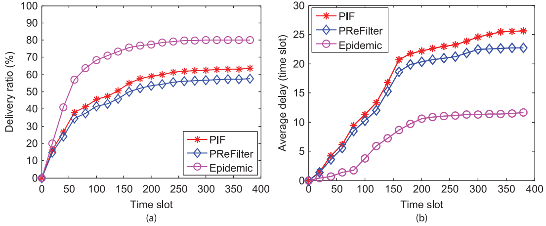
Fig. 5. Packet delivery comparison among different schemes. (a) Delivery ratio. (b) Average delay.
