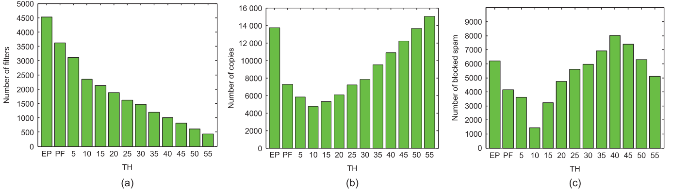
Fig. 7. Performance comparison of PIF with different THs. (a) Number of filters versus TH. (b) Number of copies versus TH. (c) Number of blocked packets versus TH.
