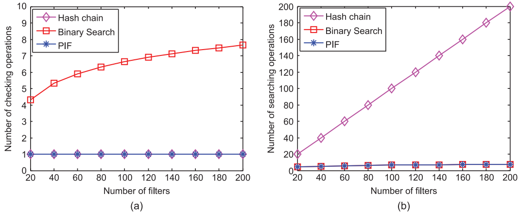
Fig. 8. Update comparison among different schemes. (a) Checking comparison. (b) Searching comparison.
