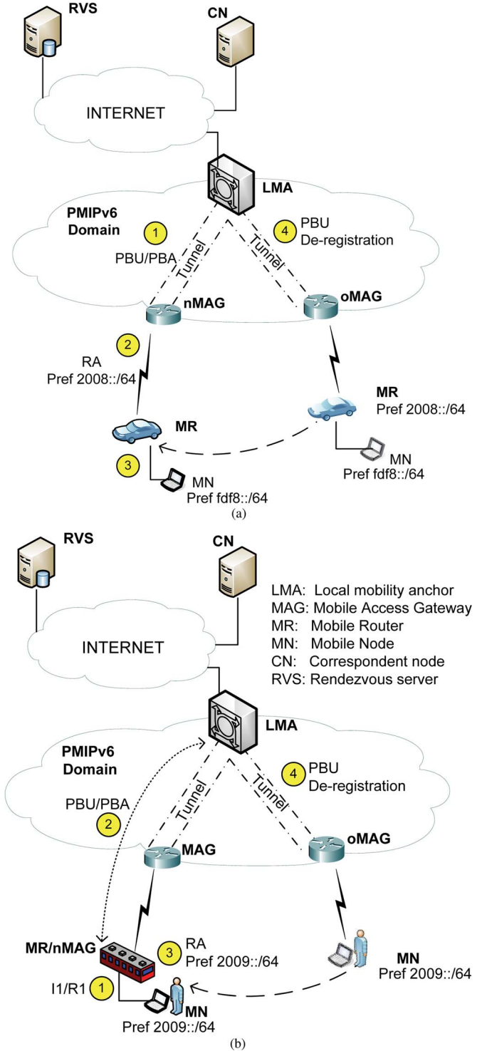
Fig. 4. Intra-domain handover in the proposed hybrid scheme. (a) Legacy node intra-domain handover. (b) HIP-enabled node intra-domain handover to a MR.
