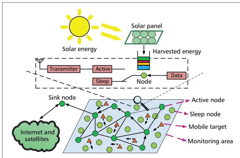
Figure 1. Energy harvesting wireless sensor network.
