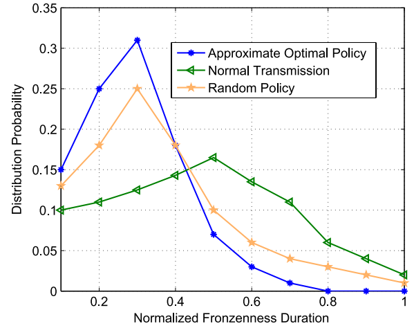
Fig. 6. Probability distribution of frozenness duration.
