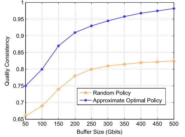
Fig. 5. Quality consistency of different buffer sizes.
