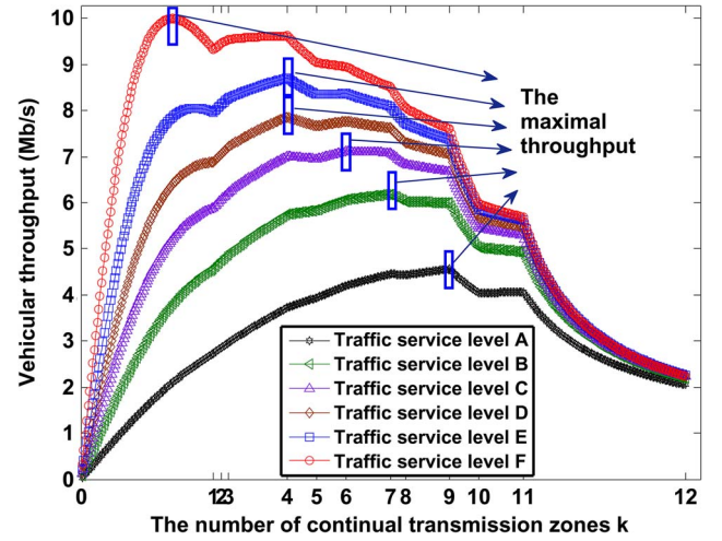
Fig. 13. The average vehicular throughput of 802.11g networks under different number of continual transmission zones.
