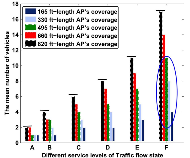
Fig. 8. The mean contending vehicular number under different Traffic flow states.
