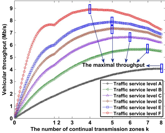
Fig. 11. The average vehicular throughput of 802.11a networks under different number of continual transmission zones.
