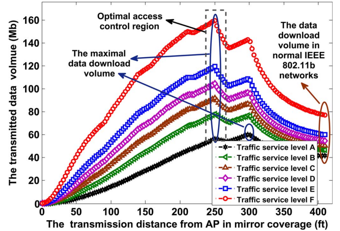
Fig. 16. The average transmitted data volume of 802.11g networks under different access control regions.
