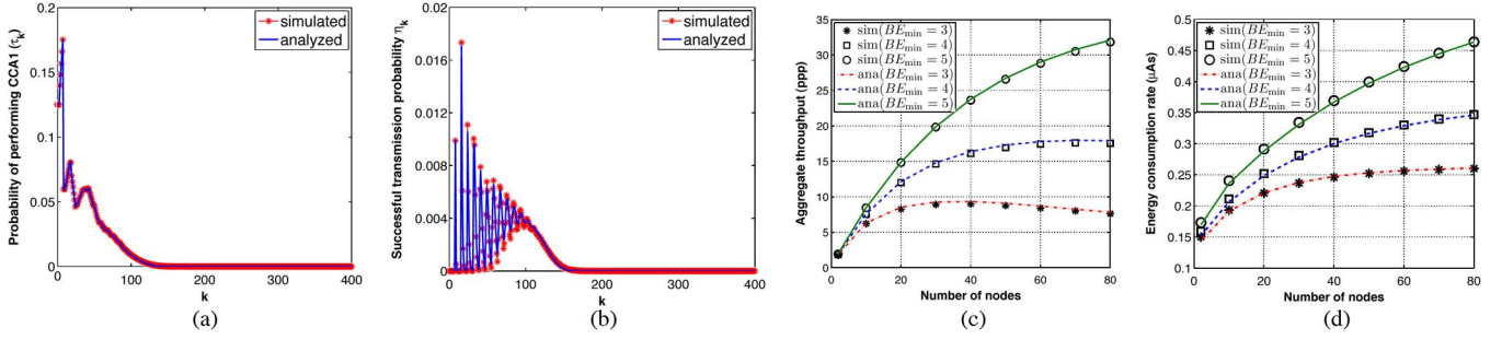
Fig. 6. MAC performance when with re-initialization ($C = 5$) but without retransmission ($R = 0$). In (a) and (b), $BE_{min} = 3, BE_{max} = 5$. (a) Probability of performing CCA1 ($\tau_k$). (b) Successful transmission probability $\eta_k$. (c) Aggregate throughput. (d) Energy consumption rate ($\mu As$).
