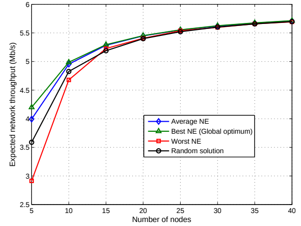
Fig. 10. Performance comparison for different solutions in terms of the achieved network throughput in small networks ( \theta=0.6 ).
