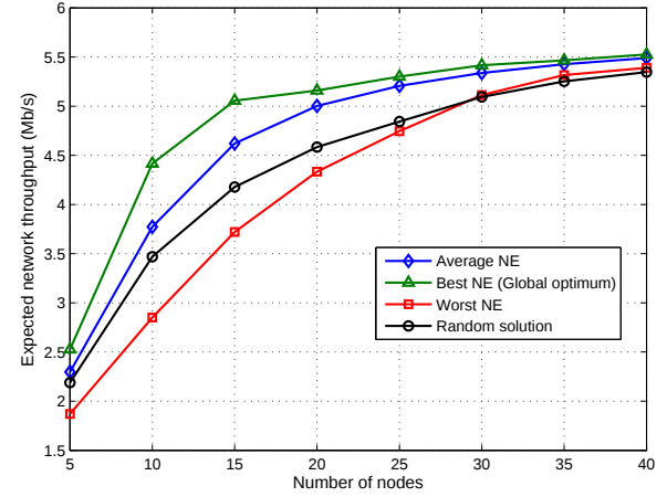
Fig. 11. Performance comparison for different solutions in terms of the achieved network throughput in small networks ( \theta varies for different nodes).
