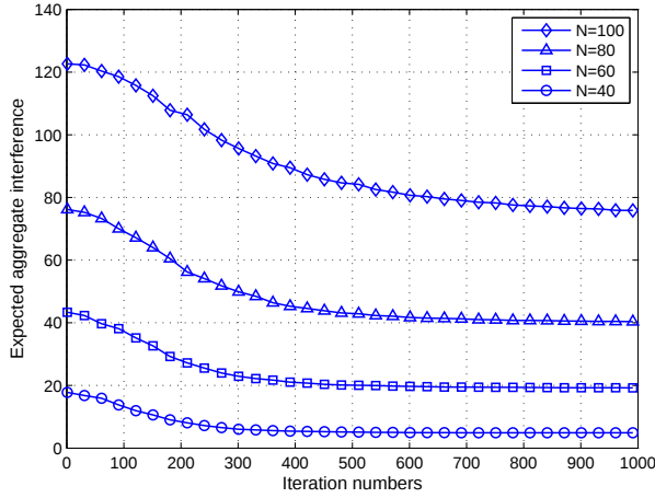
Fig. 6. Convergence comparison for different numbers of nodes ( \theta=0.6 ).
