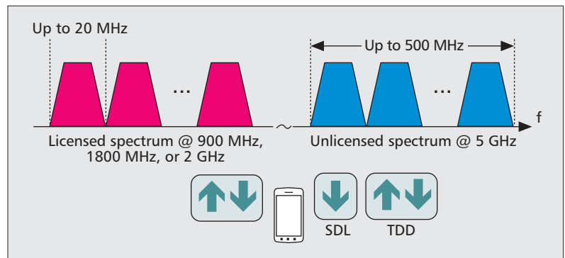
Figure 2. Two LTE-U operation modes: supplemental downlink (SDL) and TDD [5].
