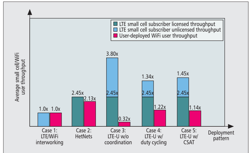
Figure 6. Average user throughput comparisons in both licensed and unlicensed spectrum under different deployment patterns.
