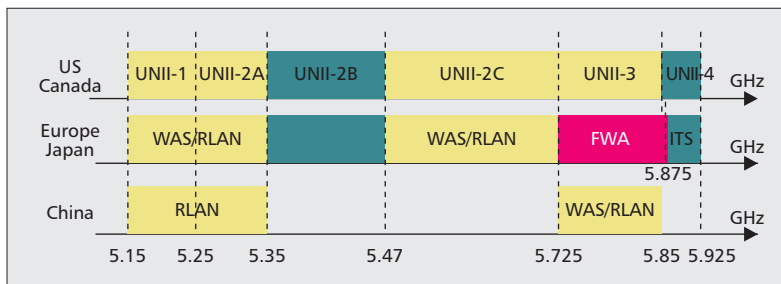
Figure 1. Unlicensed spectrum layout in different main regions at 5 GHz.
