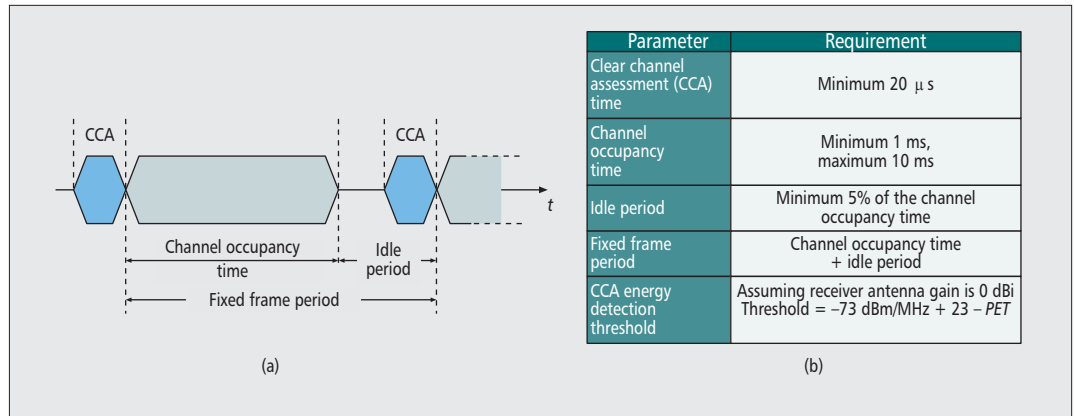
Figure 4. ETSI specifications on LBT time-based frame structure [8]: a) ETSI LBT frame structure; b) key parameters of the frame structure.
