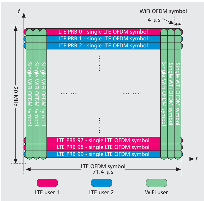
Figure 3. PHY and MAC comparisons between LTE and WiFi systems in both time and frequency domains [9]. For a 20 MHz LTE channel (one carrier), its effective transmission bandwidth is 18 MHz. One PRB is 180 kHz. Thus, a 20 MHz LTE channel has 100 PRBs, which can be allocated to multiple users (users 1 and 2) simultaneously. In contrast, all the bandwidth in a WiFi system can only be occupied by one user within each 4 μs OFDM symbol.
