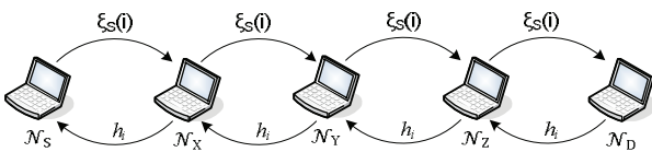
Fig. 2: The exchanged cryptographic tokens during data transmission.
