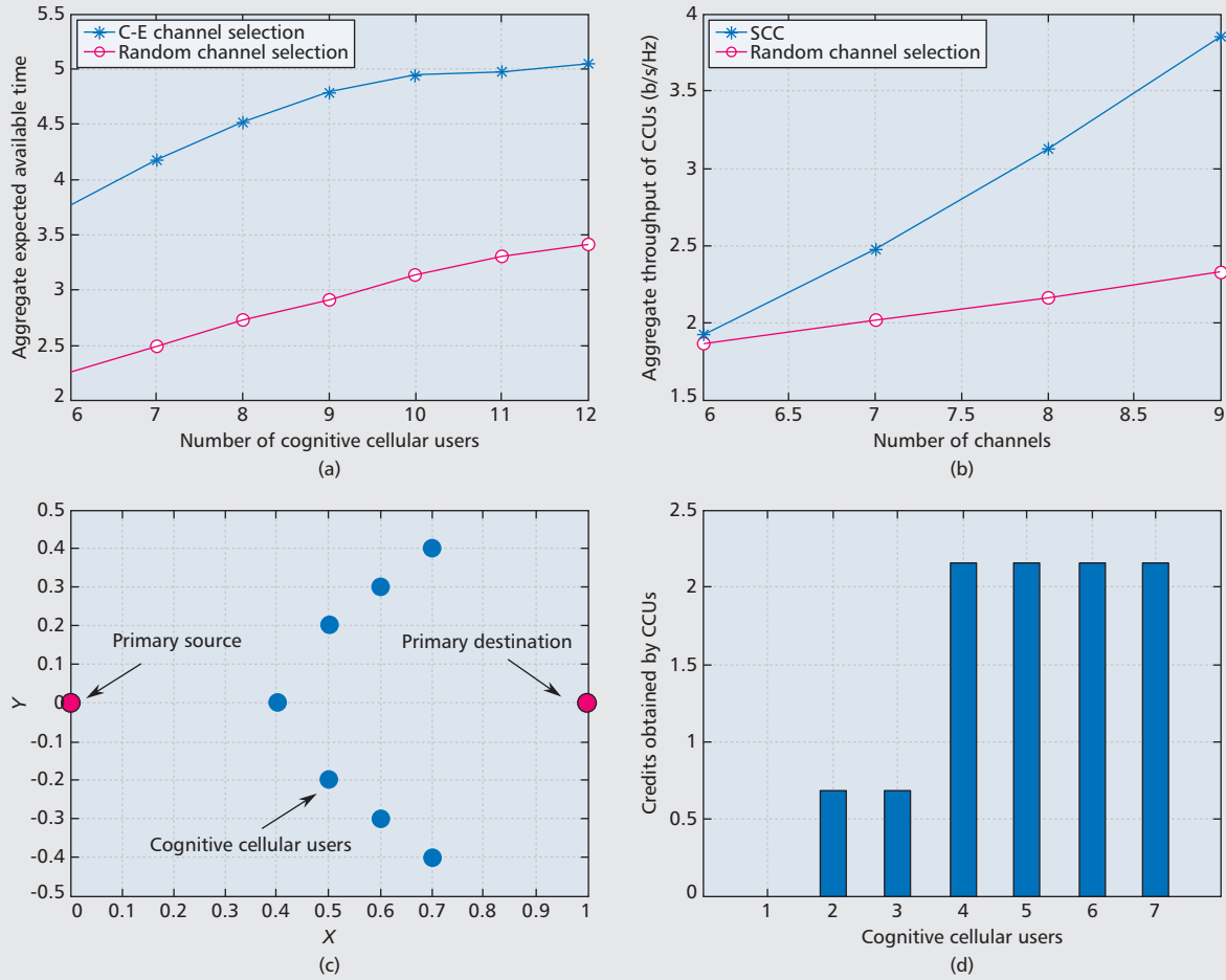
Figure 4. Performance of the cooperation based spectrum harvesting schemes: a) aggregate expected available time vs. number of CCUs; b) aggregate throughput vs. the number of channels; c) network scenario for simulation; d) credits earned by CCUs through cooperation.
