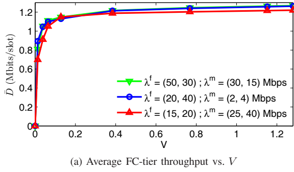
Fig. 3. Average FC-tier throughput and queue backlog vs. V under JACRA
