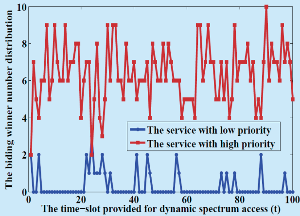
Fig.9 The winner number distribution for two prioritized services
