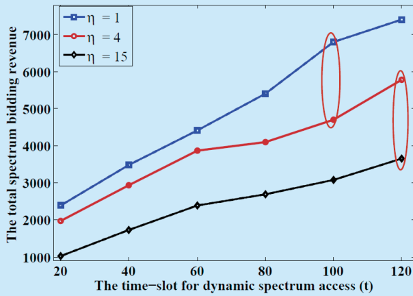
Fig.8 The spectrum trading revenue statistic with different \eta
