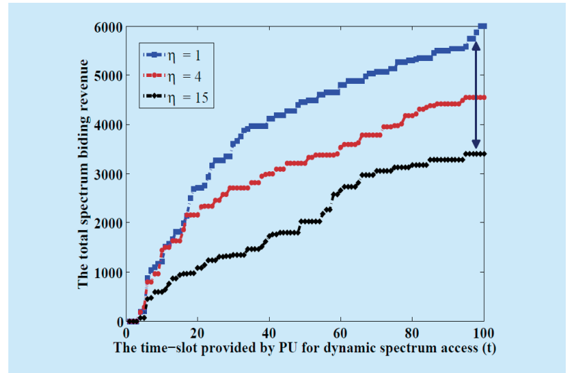
Fig.7 The tracking of spectrum trading revenue with different \eta
