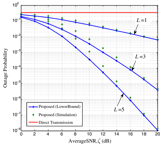
Figure 7. Outage probability of the proposed scheme for target bit error rate of 10^{-3} and different values of L .
