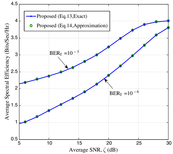
Figure 5. Comparison between the average spectral efficiency of the proposed scheme using Equation 13 and its approximation in Equation 14 for L = 3 and for two different target bit error rates (BERs).
