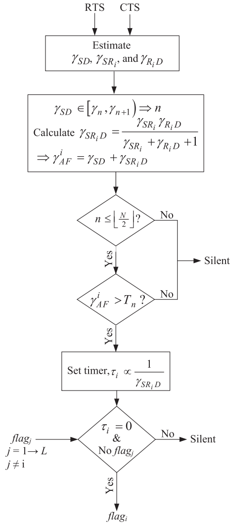
Figure 3. Flow chart of the proposed scheme at the relay node, R_i, i = 1, 2, \dots, L .
