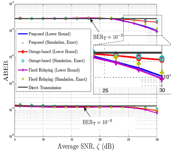
Figure 6. Average bit error rate (ABER) of the proposed scheme, the outage-based, the fixed relaying, and the direct transmission for L = 1 , and for two different target BERs.
