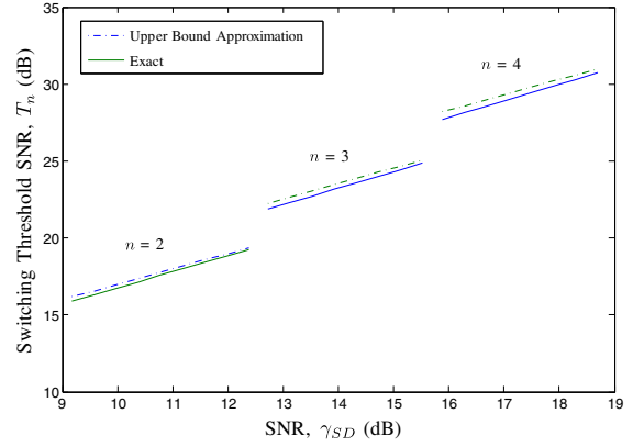
Figure 2. Switching threshold signal-to-noise ratio (SNR), T_n , and its upper bound approximation.
