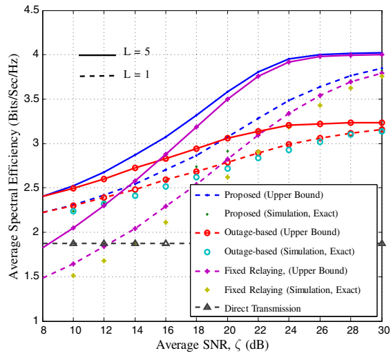
Figure 4. Average spectral efficiency of the proposed scheme, outage-based, fixed relaying, and the direct transmission for target bit error rate of 10^{-3} and different values of L .
