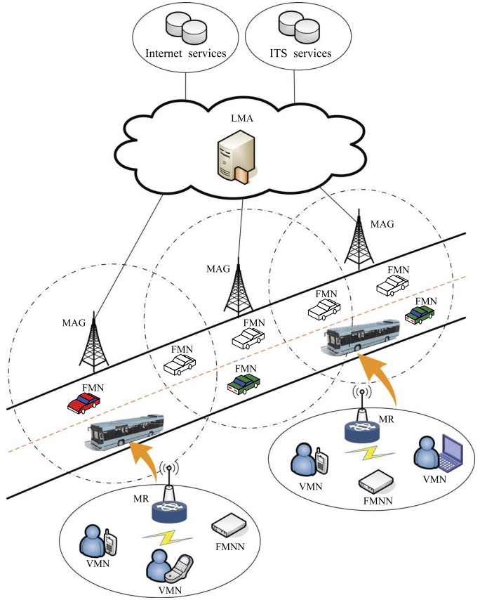
Fig. 1. Architecture of a localized E-PMIPv6 domain.
