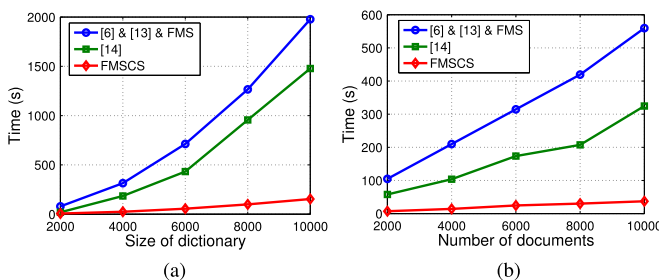
Fig. 6. Time for building index. (a) For the different size of dictionary with the same number of documents, N = 6,000 . (b) For the different number of documents with the same size of dictionary, |\mathcal{W}| = 4,000 .
