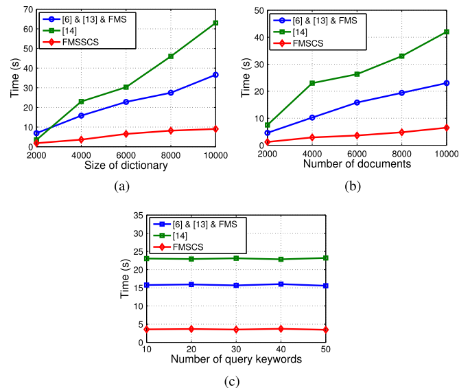
Fig. 8. Time for query. (a) For the different size of dictionary with the same number of documents and number of search keywords, N = 6,000 , |\mathcal{W}| = 20 . (b) For the different number of documents with the same size of dictionary and number of search keywords, |\mathcal{W}| = 4,000 . (c) For the different number of search keyword with the same size of dictionary and number of documents, N = 6,000 , |\mathcal{W}| = 4,000 .
