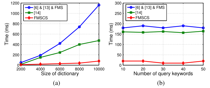
Fig. 7. Time for generating trapdoor. (a) For the different size of dictionary with the same number of query keywords, |\mathcal{W}| = 20 . (b) For the different number of query keywords with the same size of dictionary, |\mathcal{W}| = 4,000 .
