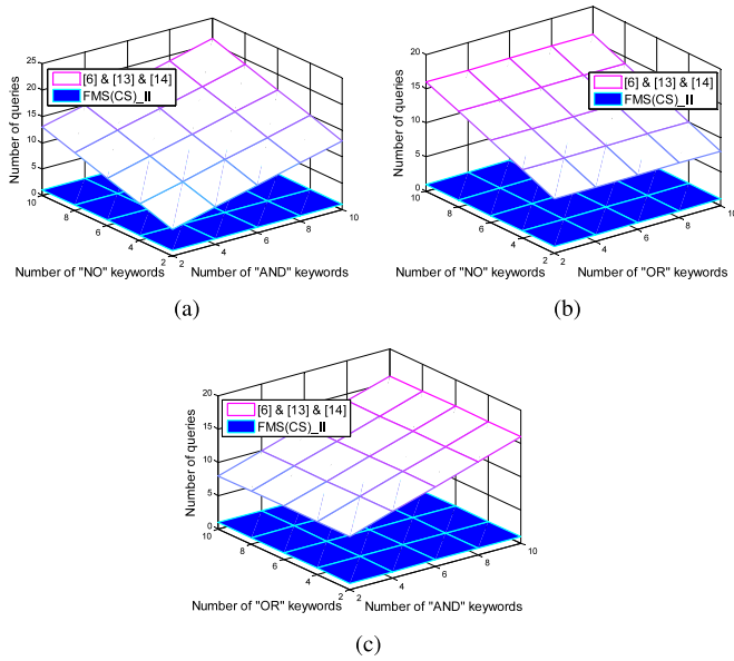
Fig. 5. Query complexity. (a) Number of queries for the different number of “AND” and “NO” keywords with the same number of “OR” keywords, l_1 = 5 . (b) Number of queries for the different number of “OR” and “NO” keywords with the same number of “AND” keywords, l_2 = 5 . (c) Number of queries for the different number of “AND” and “OR” keywords with the same number of “NO” keywords, l_3 = 5 .
