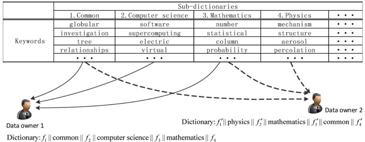
Fig. 4. Classified sub-dictionaries.
