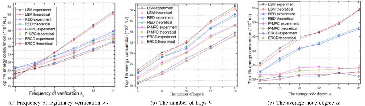
Fig. 12. Top 1 percent Energy consumption of ERCD or existing protocols under different parameters.
