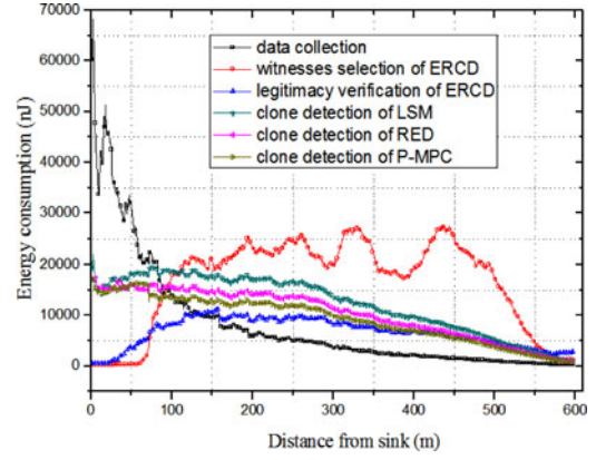
Fig. 11. Energy consumption of each step by using ERCD or existing protocols.
