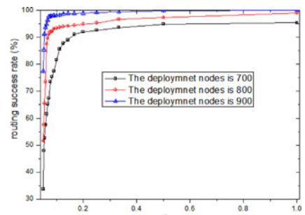
Fig. 15. Routing success rate with various duty cycle.
