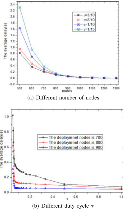
Fig. 16. Average delay by using ERCD protocol.
