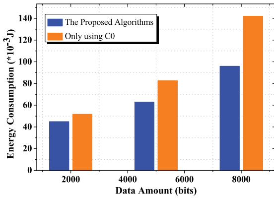
Fig. 10. Total energy consumption comparison under different amount of data traffic.
