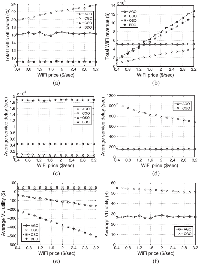
Fig. 7. Simulation results in terms of WiFi price. (a) Total traffic offloaded. (b) Total WiFi revenue. (c) Average service delay. (d) Average service delay (AGO versus CGO). (e) Average VU utility. (f) Average VU utility (AGO versus CGO).
