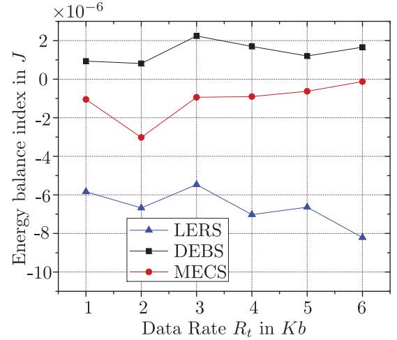
Fig. 8. Energy balance index versus data rate R_t .
