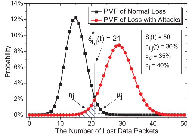
Fig. 3. An example of the optimal threshold.
