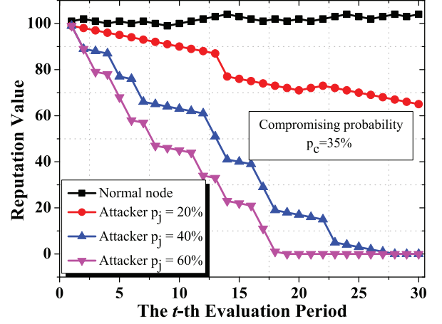
Fig. 5. Reputation value comparison.
