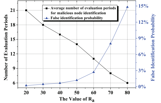
Fig. 11. The Impacts of R_a on the Performance of CRS-A.
