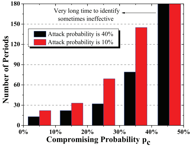
Fig. 10. CRS-A performance for different compromising probabilities.
