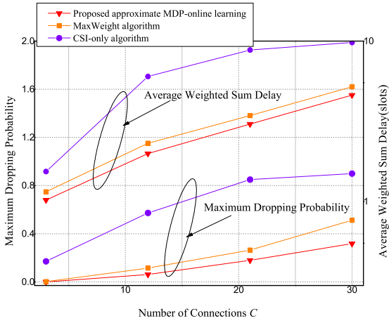
Fig. 3. The average weighted sum delay and the maximum dropping probability over all connections versus the number of connections C with \lambda = 1 packets/slot and d_{\max} = 0.3 . The number of connections is C = 3(D = C_u = C_d = 1) , C = 12(D = C_u = C_d = 4) , C = 21(D = C_u = C_d = 7) , C = 30(D = C_u = C_d = 10) , respectively.
