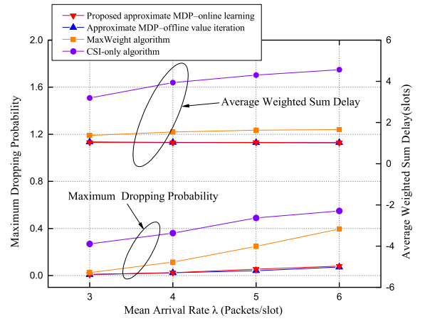
Fig. 2. The average weighted sum delay and the maximum dropping probability over all connections versus the mean arrive rate \lambda with C = 3 ( D = C_u = C_d = 1 ) and d_{\max} = 0.1 .
