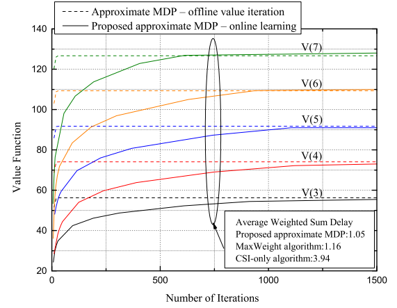
Fig. 4. Illustration of the convergence property of the proposed online stochastic learning algorithm and brute-force offline value iteration algorithm with C = 3(D = C_u = C_d = 1) and \lambda = 5 packets/slot.
