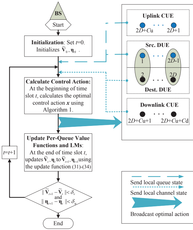
Fig. 1. The implementation flow of Algorithm 2 with online stochastic learning (solution to Problem 1).
