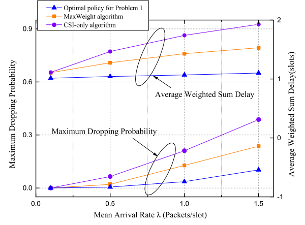
Fig. 4. The average weighted sum delay and the maximum dropping probability over all connections versus the mean arrive rate \lambda with d_{\max} = 0.1 and R = 100\text{m} .
