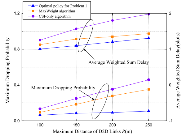
Fig. 5. The average weighted sum delay and the maximum dropping probability over all connections versus the maximum distance of D2D links R with \lambda = 1.5 packets/slot and d_{\max} = 0.1 .
