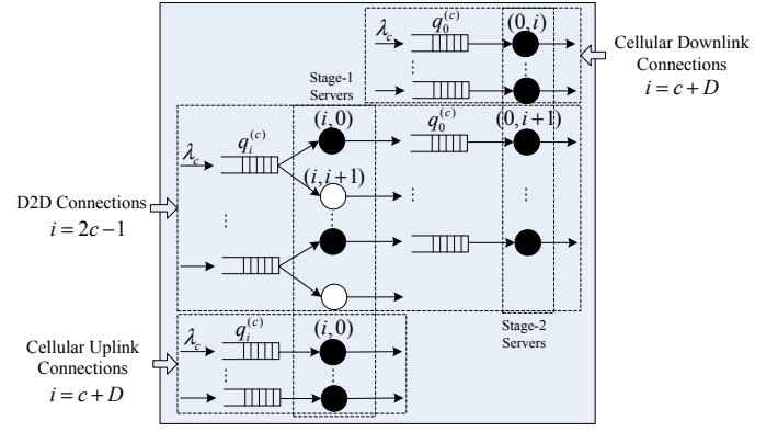
Fig. 2. Queuing model for the general network model.
