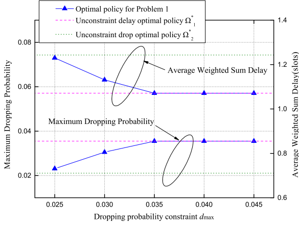
Fig. 3. The average weighted sum delay and the maximum dropping probability over all connections versus the dropping probability constraint d_{\max} with \lambda = 1 packets/slot and R = 100\text{m} .
