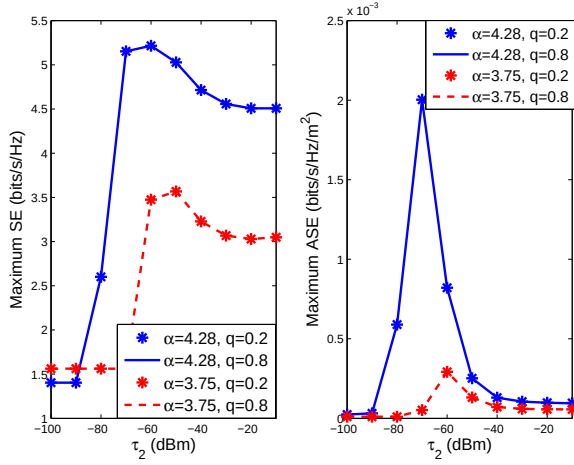
Fig. 10. The corresponding maximum SE and ASE.
