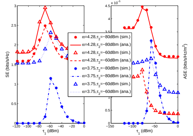
Fig. 4. SE and ASE with respect to cooperative threshold \tau_1 for different path-loss exponents and cooperative threshold \tau_2 ( q = 0.5 , D_1 = 400\text{m} , D_2 = 100\text{m} , D_3 = 20\text{m} , \tau_3 = -45\text{dBm} ).
