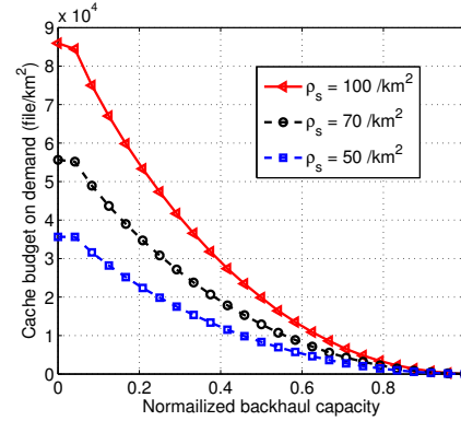
Fig. 7: Cache budget demand on different backhaul capacity.
