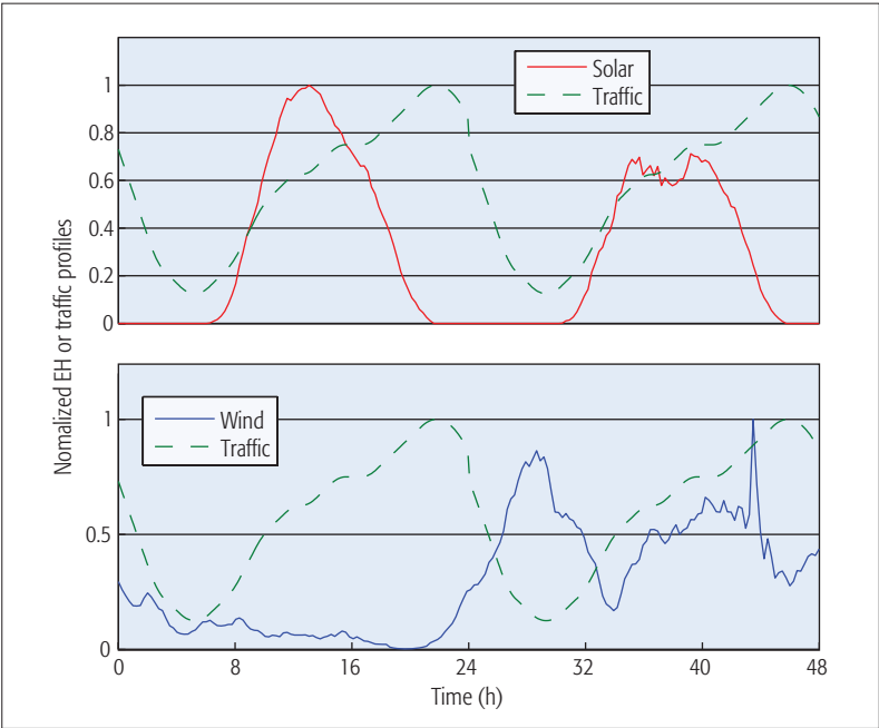
Figure 2. Daily energy harvesting and traffic demand profiles.
