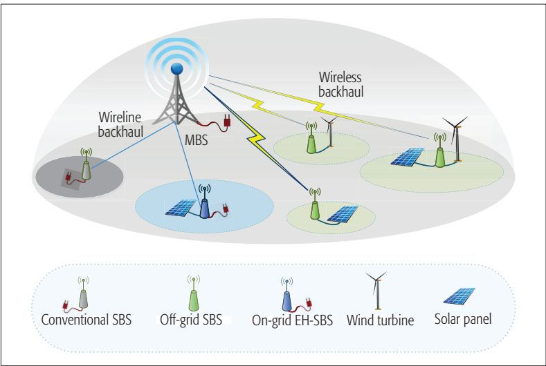
Figure 1. Network architecture with renewable energy harvesting.
