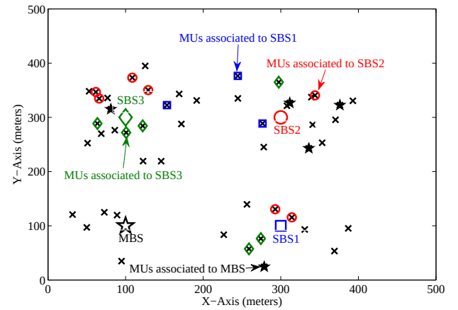
Fig. 2. The optimal SBS association obtained when maximizing the equivalent capacity (i.e., \sum_{j=1}^N \sum_{i=1}^M x_{ij} ) for the uplink SCN as in Fig. 1. Specifically, the number of MUs in service is 5, 3, 7, and 6 associated to MBS, SBS 1, SBS 2, and SBS 3, respectively.
