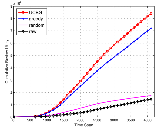
Fig. 3. Comparison of cumulative utility of the crowdsourcing platform.
