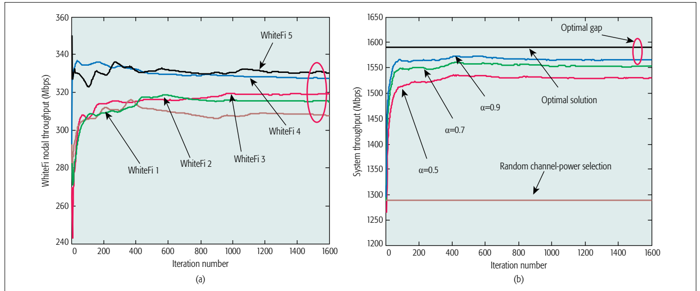
FIGURE 6. Distributed Markov approximation based dynamic TV white space planning: a) the average WhiteFi nodal throughput with 2-frequency configuration; b) the average WhiteFi network throughput with 10 nodes and single-frequency configuration.
