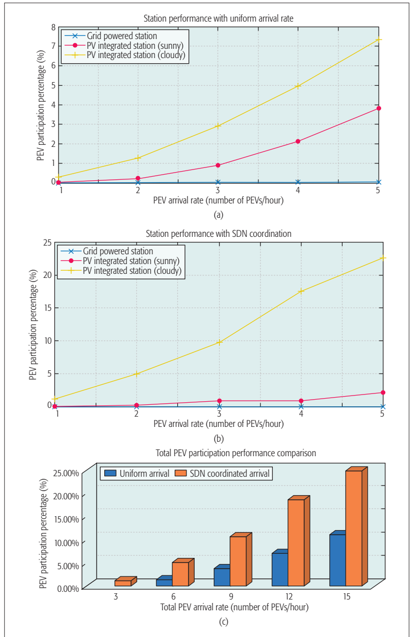
FIGURE 6. The Station Ancillary Service Performance.
