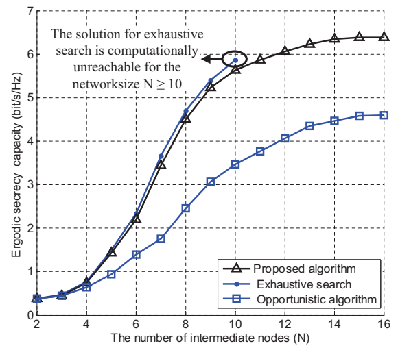
Fig. 7. Performance comparison in terms of secrecy ergodic capacity between Algorithm 2, opportunistic selection and exhaustive searching.
