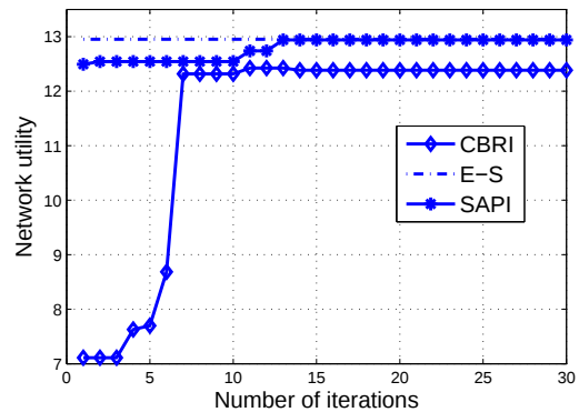
Figure 6. Convergence of the proposed algorithms.
